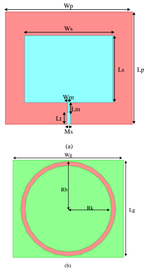
Fig 1. Structure of Directional 1900 MHz Square Patch Ring Slot Microstrip Antenna (a) Front, (b) Rear
