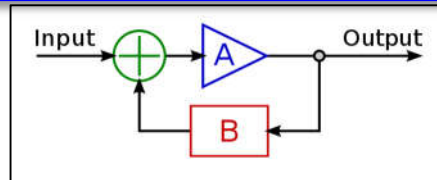
Fig. 3. Ideal Feedback of Schmitt trigger
