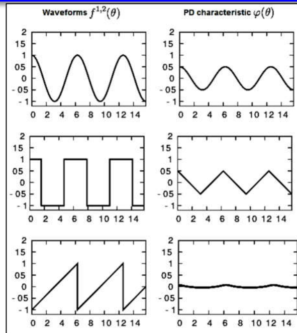
Fig. 2. Phase Detector Multiplier Characteristic
