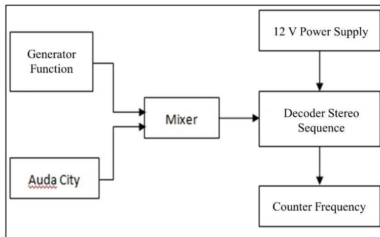
Fig. 6.. Block Diagram of DSB-SC Demodulator Testing
