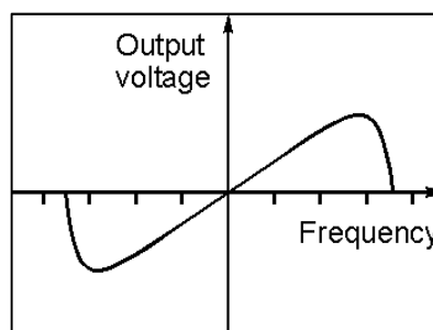
Fig. 1. "S" Curve Characteristic in FM Demodulator
