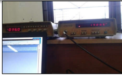
Fig. 7. Frequency Result of R Audio Channel in 36 kHz Frequency
