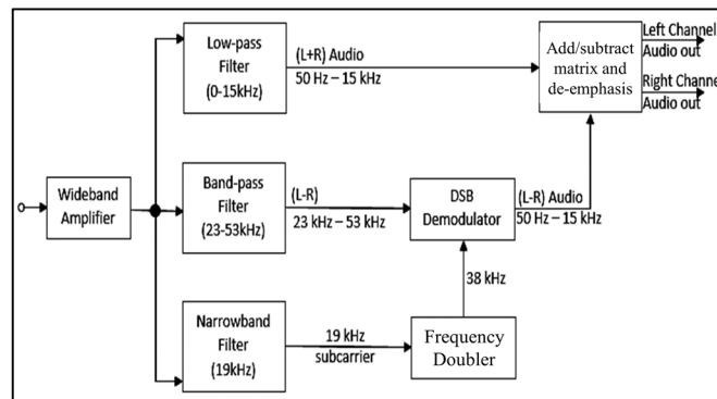
Fig. 4. System Block Diagram
