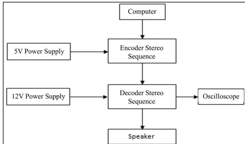
Fig. 9.. Block Diagram of Encoder to Decoder Testing
