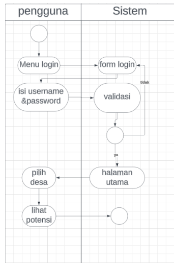
Gambar 4. Flowchart Sistem
