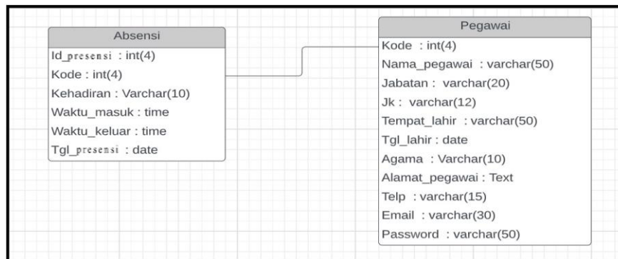
Gambar 9. Class diagram
