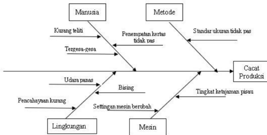
Gambar 5. Diagram Fishbone
