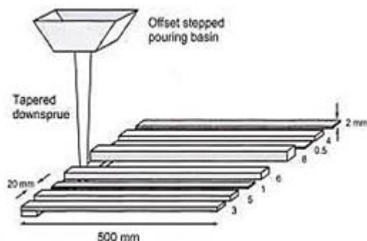
Gambar 14. Saluran Tuang Model Offset Stepped Basin Sumber: Sugeng Slamet, 2017
